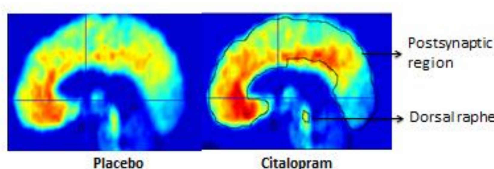
Figure 3: The [ 11 C]CUMI-101 summed BP ND parametric PET image of a representative subject showing citalopram-induced increases in 5-HT 1A receptor availability in the postsynaptic brain region
